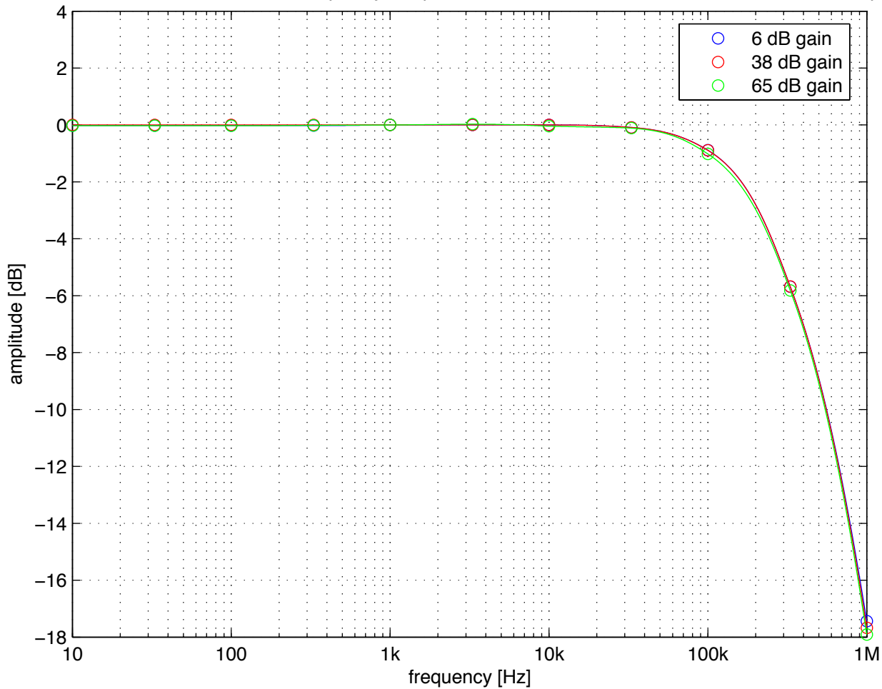
Monte Generoso Normalised Frequency Response, V_{out} = 4 \text{ V}_{rms} , R_{source} = 50 \text{ Ohm} , R_{load} = \text{open}
