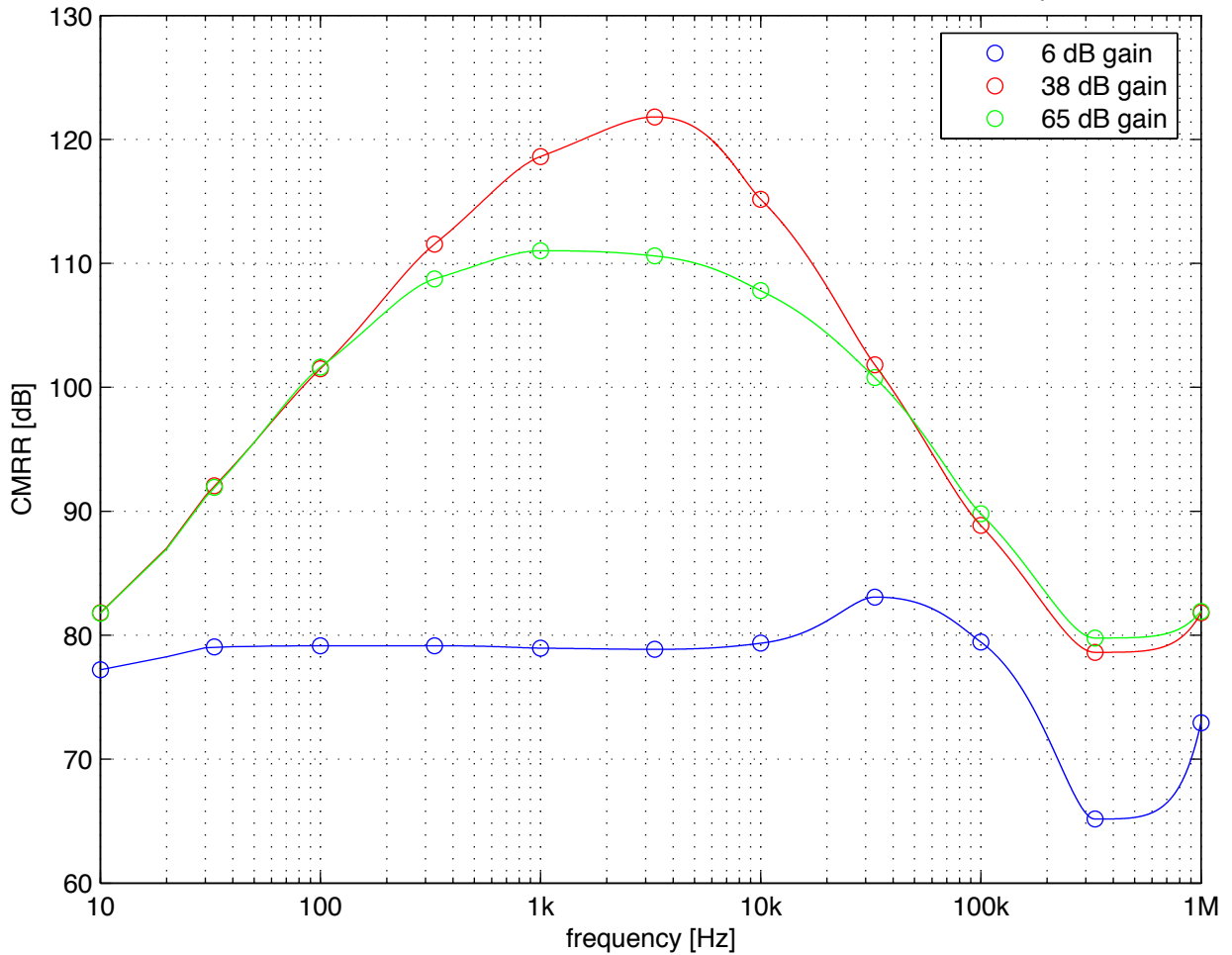
Monte Generoso CMRR, V_{in} = 4 \text{ V}_{rms} , R_{source} = 50 \text{ Ohm} , R_{load} = \text{open}
